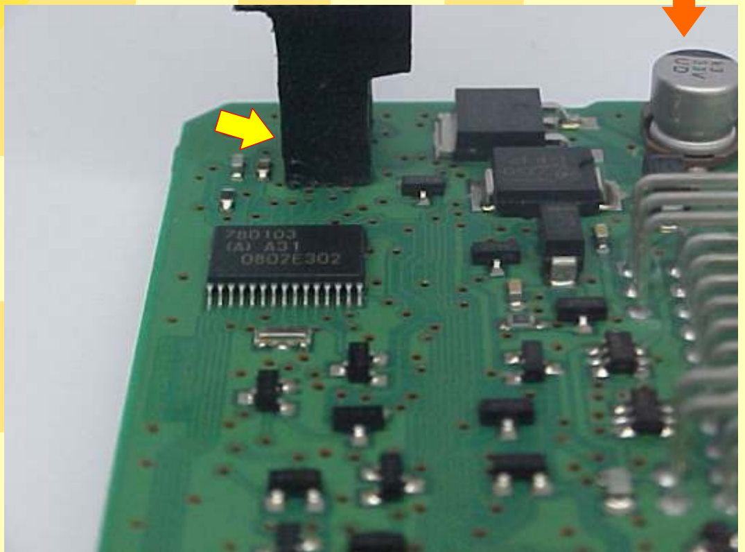
Conectando a Pinça Soic 8 na EEPROM serial 93C56
